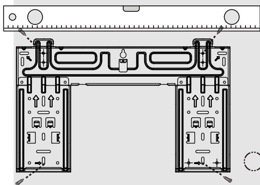
Attach Mounting Plate
